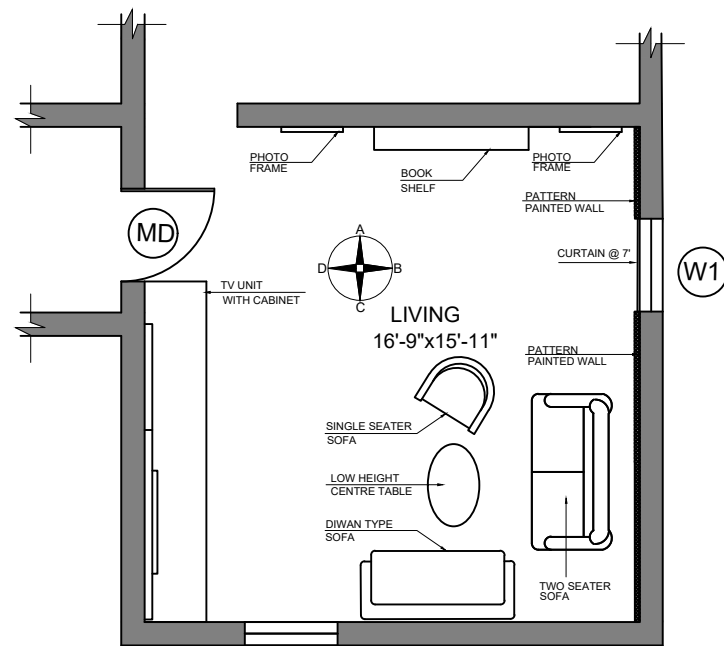
PART PLAN
