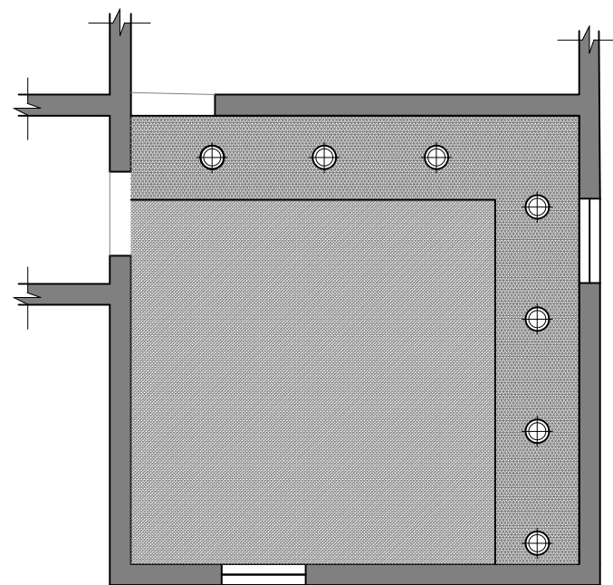
FALSE CEILING LAYOUT
