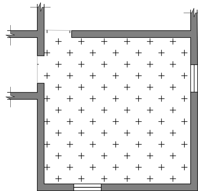
FLOORING LAYOUT
