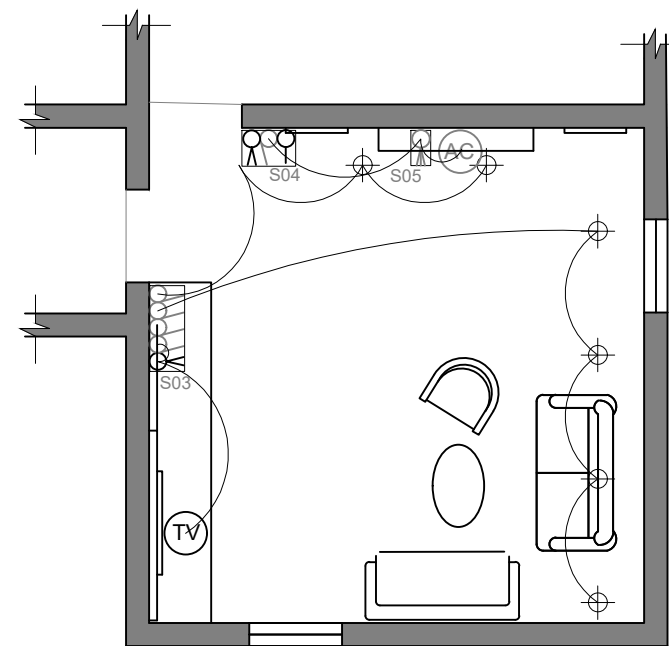
ELECTRICAL LAYOUT
