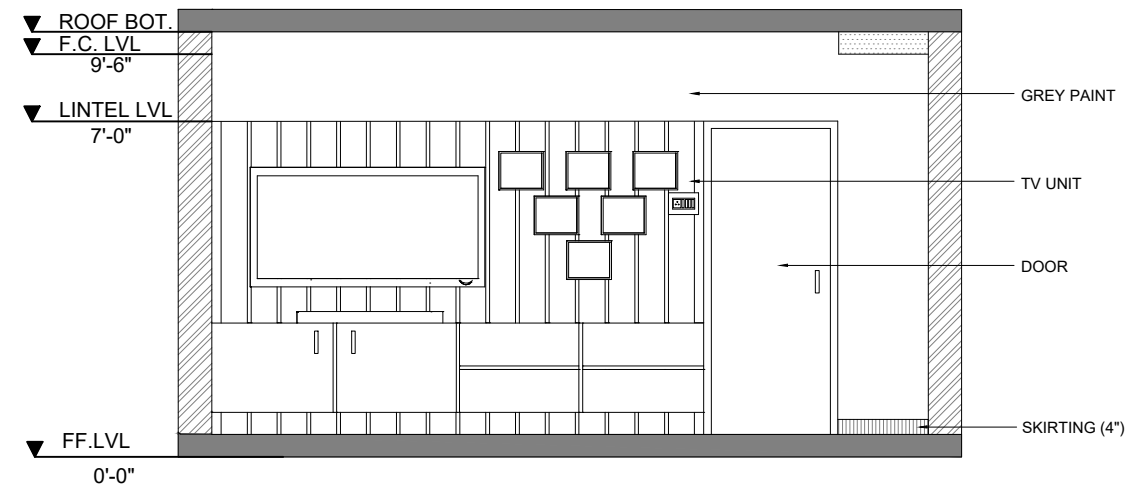
WALL - D
