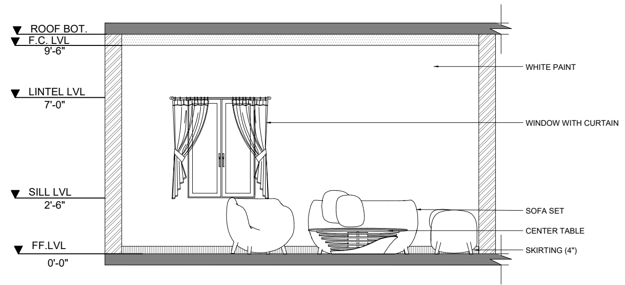
WALL - B
