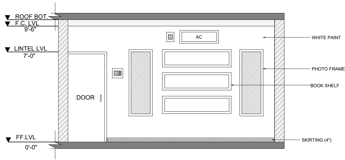
WALL - A
