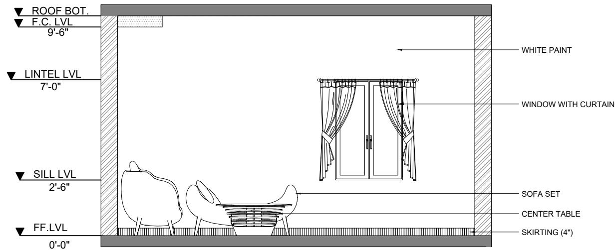
WALL - C
