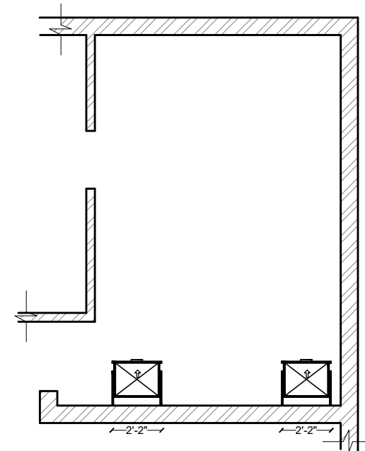
PART PLAN @1'-6" LVL
