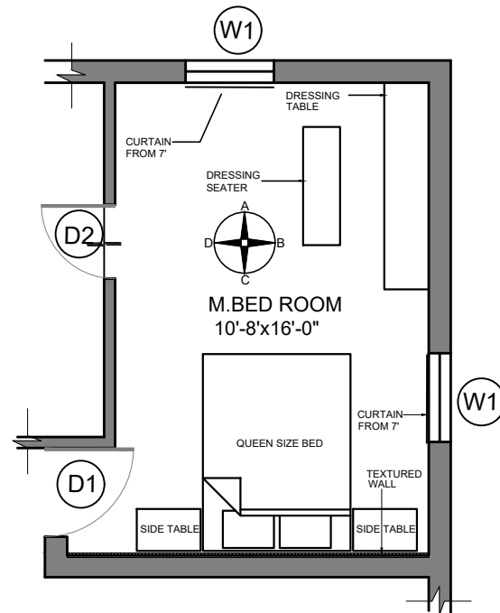
PART PLAN
