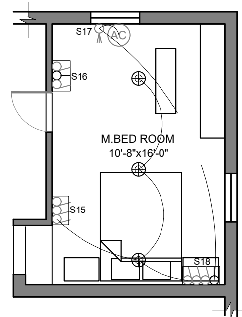
ELECTRICAL LAYOUT
