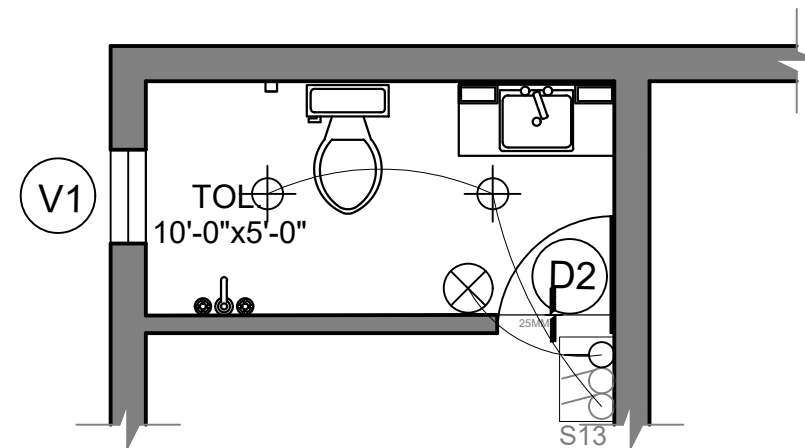
ELECTRICAL LAYOUT
