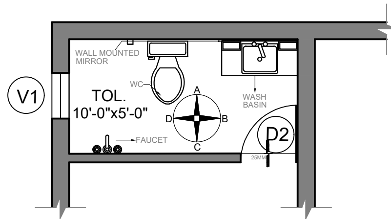
PART PLAN
