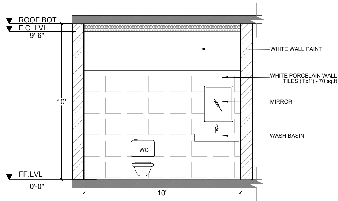
WALL - A
