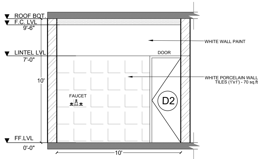
WALL - C
