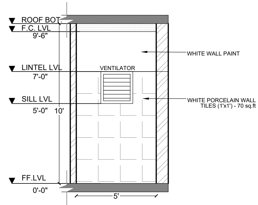
WALL - D
