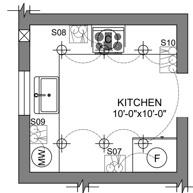
ELECTRICAL LAYOUT
