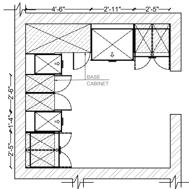
PART PLAN @2'-4"
