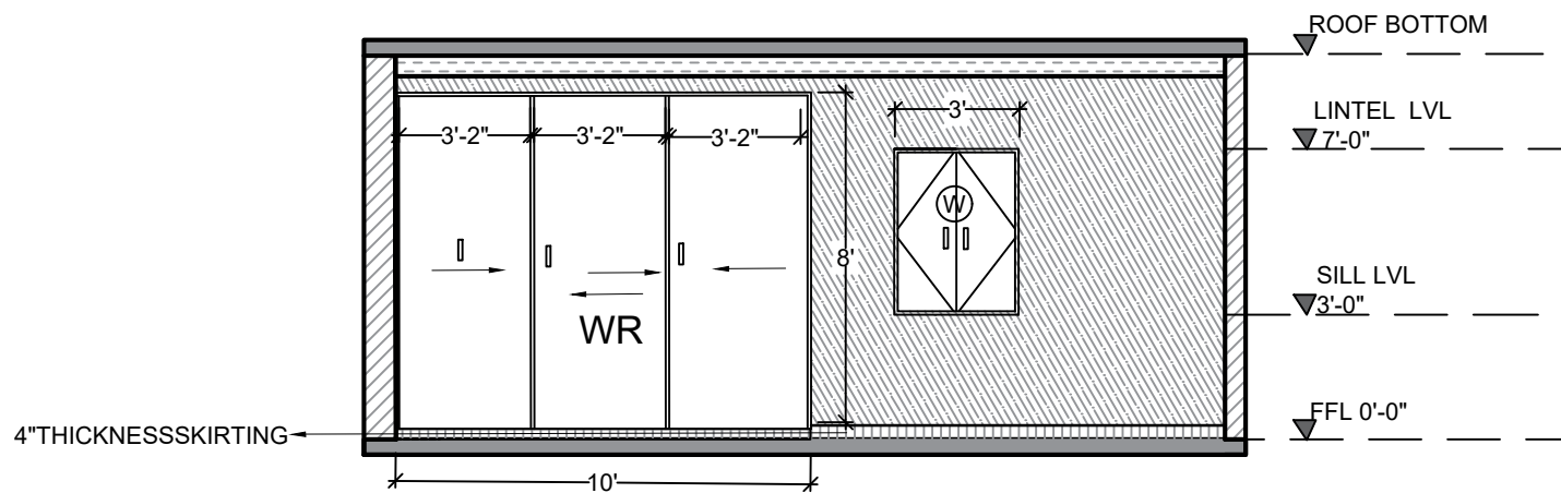
WALL ELEVATION B
