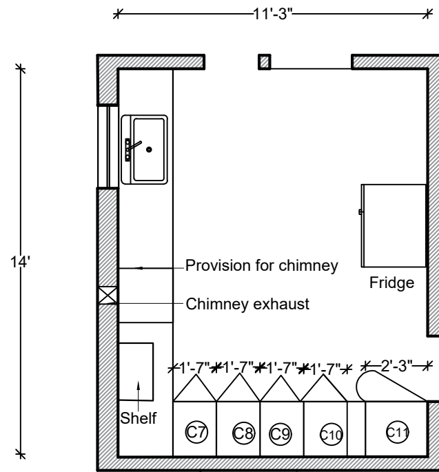
KITCHEN PART PLAN @7'-0" LVL
