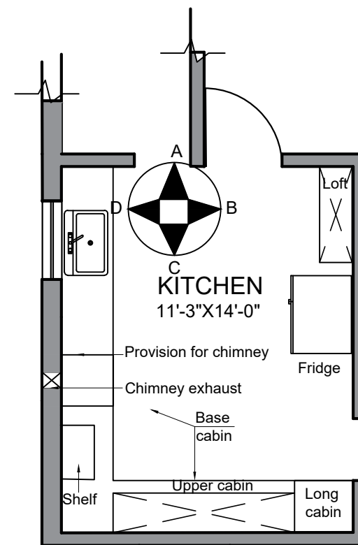
KITCHEN PART PLAN
