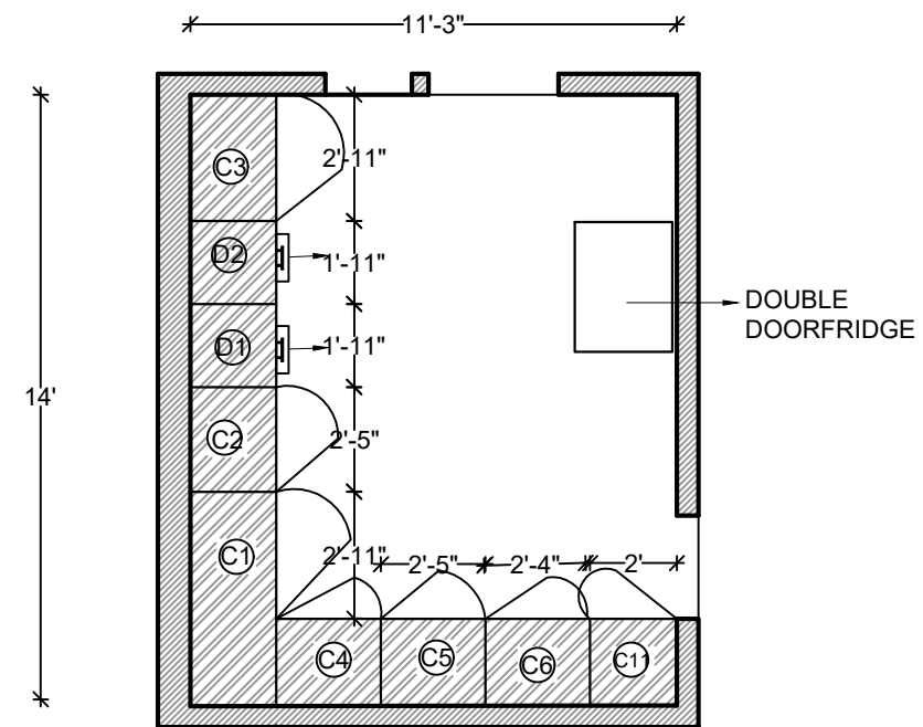
KITCHEN PART PLAN @2'-0" LVL
