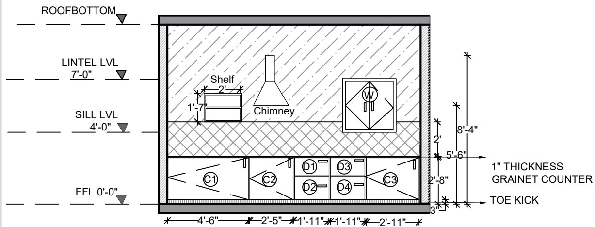
WALL ELEVATION D
