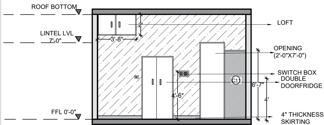
WALL ELEVATION B
