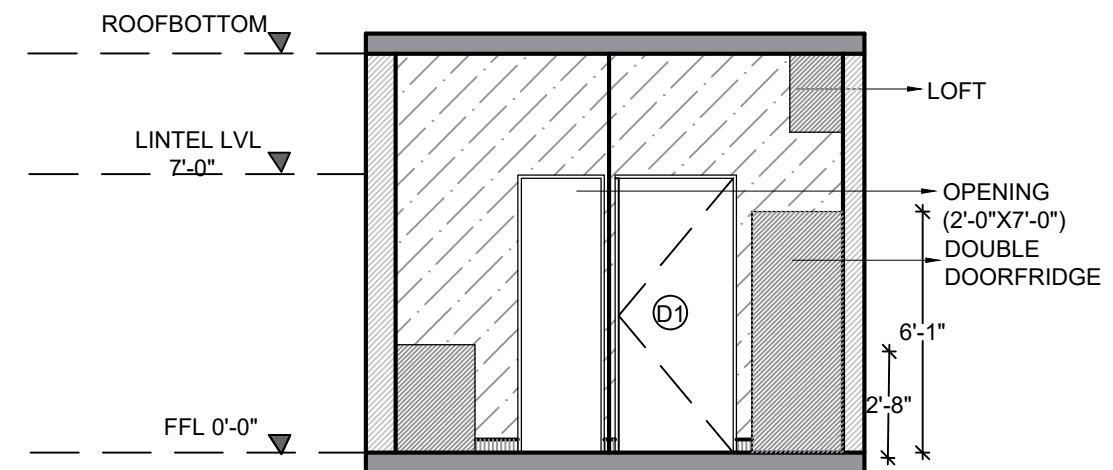
WALL ELEVATION A
