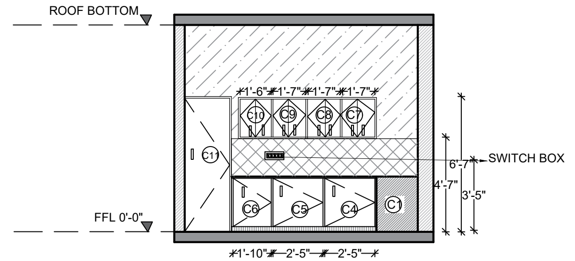
WALL ELEVATION C
